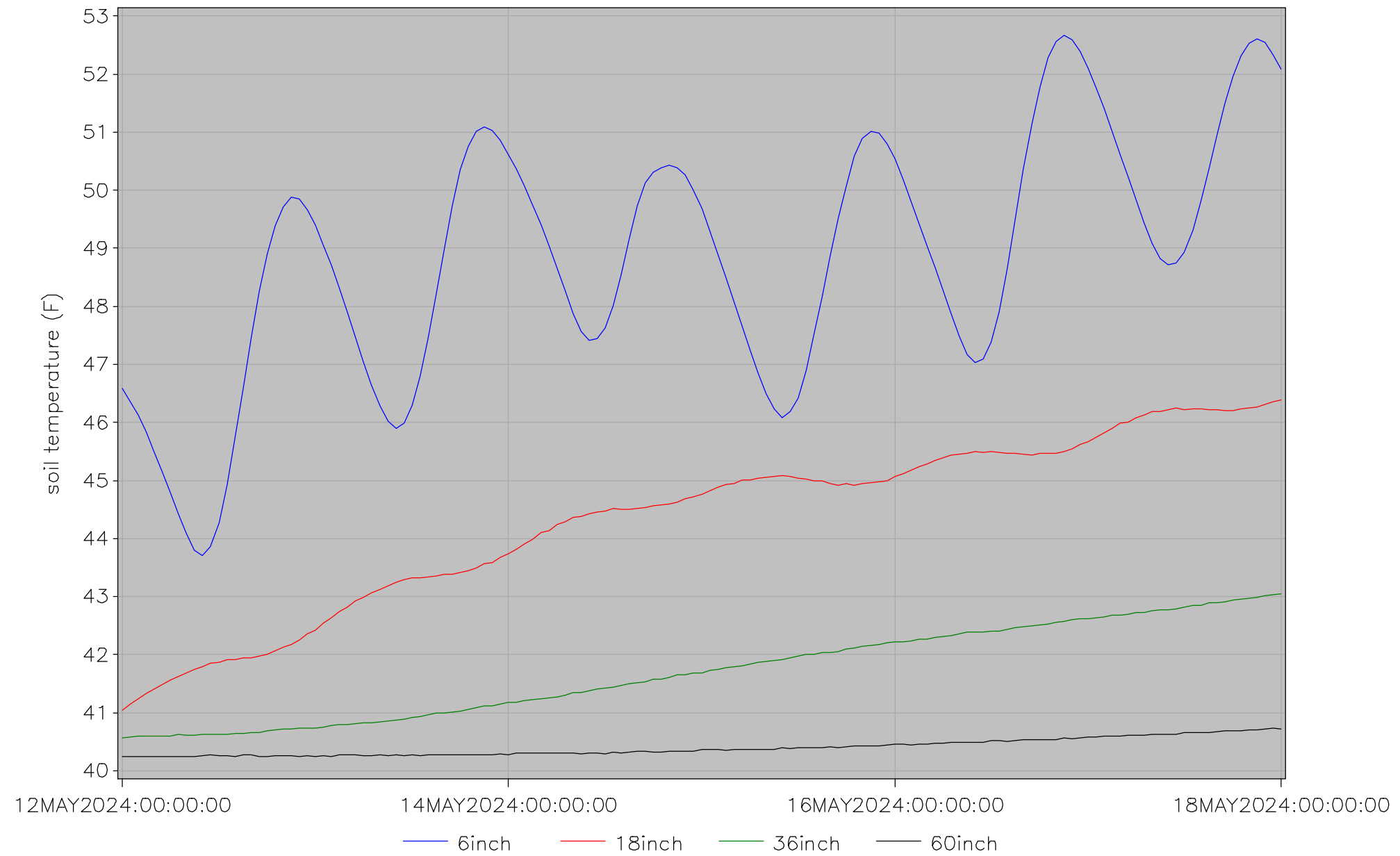
Hourly Average Soil Temperatures for the Week location=north100
