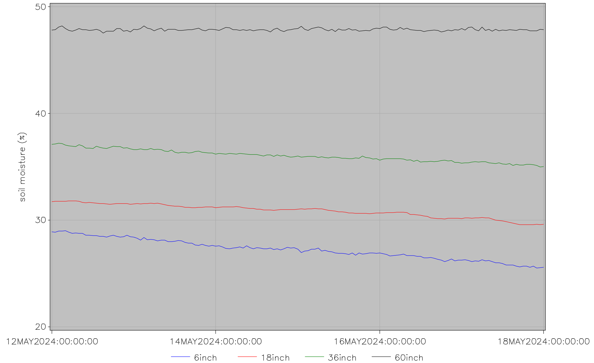
Hourly Average Soil Moistures for the Week location=north100
